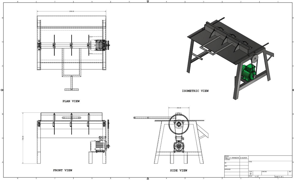
Figure 2. Orthographic view of the 3-blade cassava cutting machine
