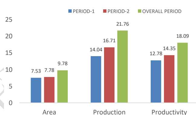
Fig-3 Magnitude of cotton area , production and productivity instability
