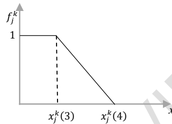
Fig. 4 lower limit measure possibility function
