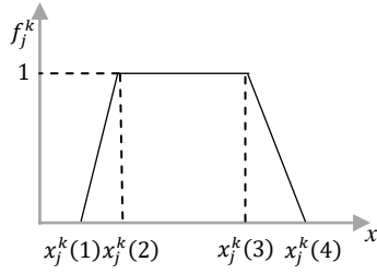
Fig. 1 typical possibility function
