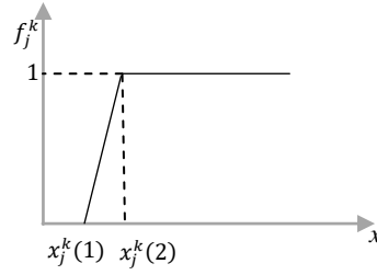
Fig. 2 upper limit measure possibility function
