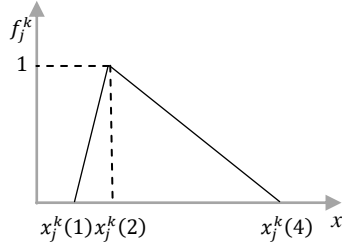
Fig. 3 moderate measure possibility function
