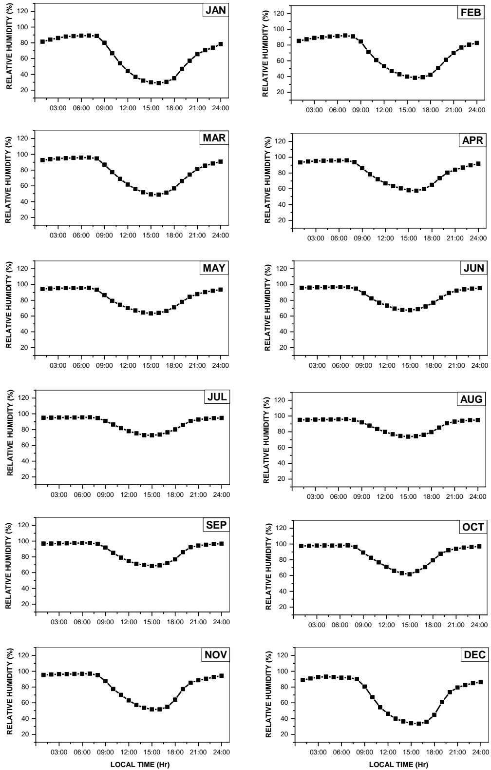
Fig. 3: Diurnal Variation of Monthly Mean Relative Humidity
