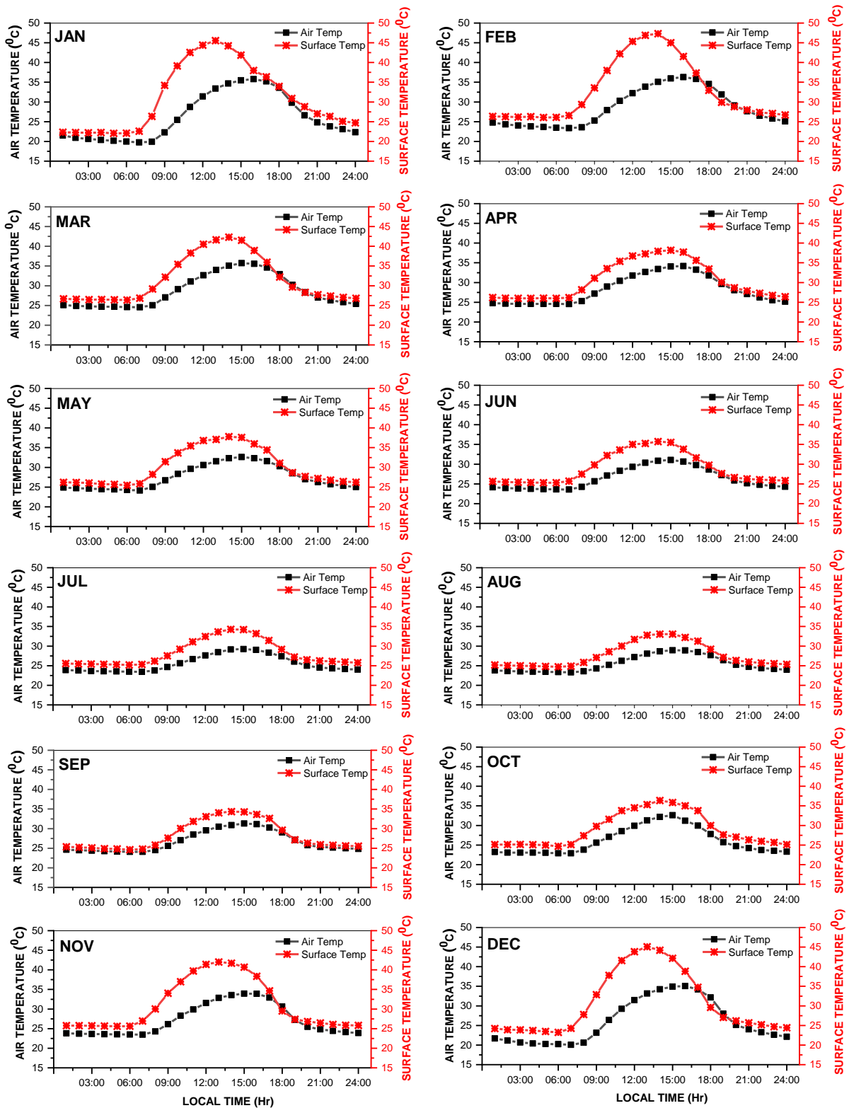
Fig. 2: Diurnal Variations of Monthly Mean Air Temperature and Surface Temperature
