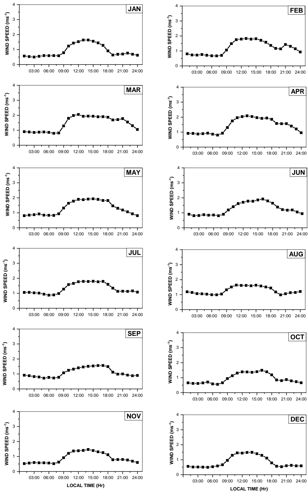
Fig. 4: Diurnal Variation of Monthly Mean Wind Speed
