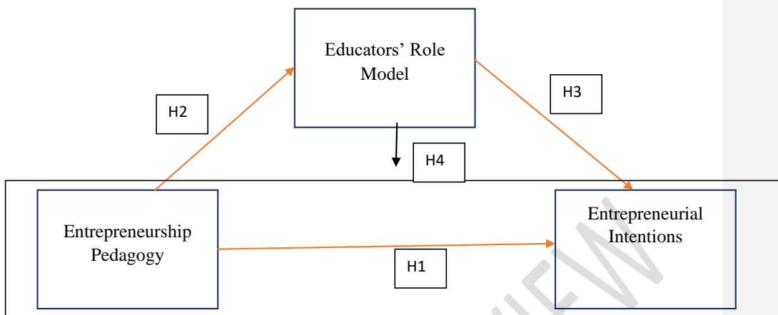
Figure 1: Conceptual Model
