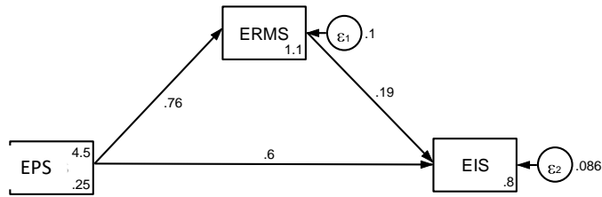
Figure 2 = SEM Model
