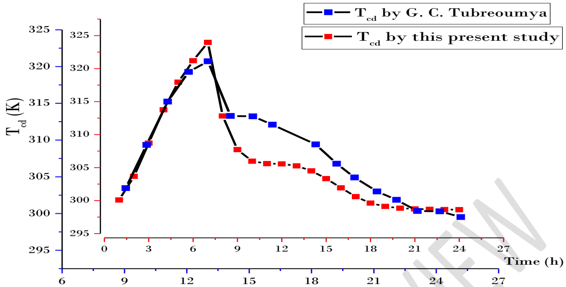
Figure 5: Condenser validation.
