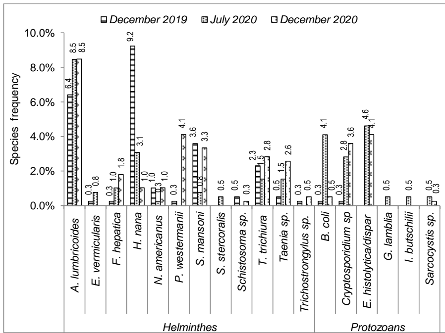
Figure 2: Frequencies of helminth and protozoan species identified in human samples in 2019 (November-December) and 2020 (July-August, November-December)
