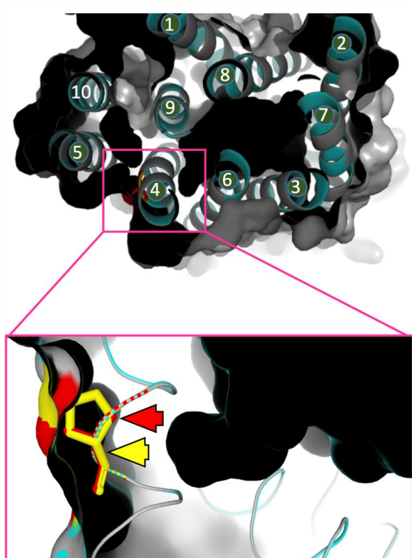
Figure 4. PfCRT homology modeling with P-165-A substitution in mut-PfCRT. The homology modeling of PfCRT was done based on PfCRT-7G8-Pro165 TMD's crystal structure (PDB 6UKJ). In blue are the TMDs of mut-PfCRT-7G8 overlapping with the gray TMDs of mut-P165A-PfCR ETSE . In yellow is the proline (yellow arrow) and in red is the alanine (red arrow).
