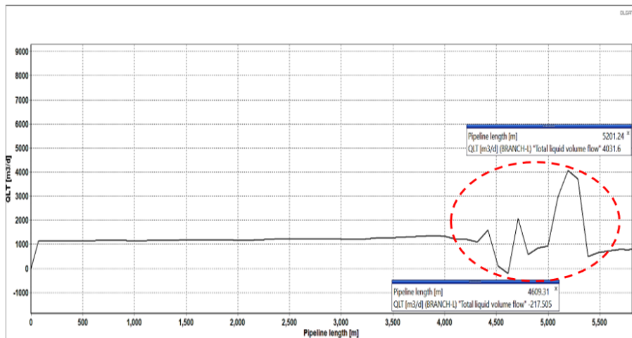
Figure 7. Total Liquid Volume Flow profile at 30,000s
