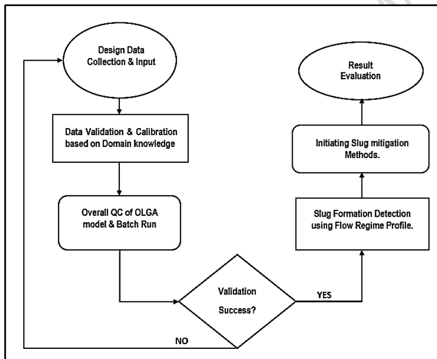
Figure 23: OLGA Workflow
