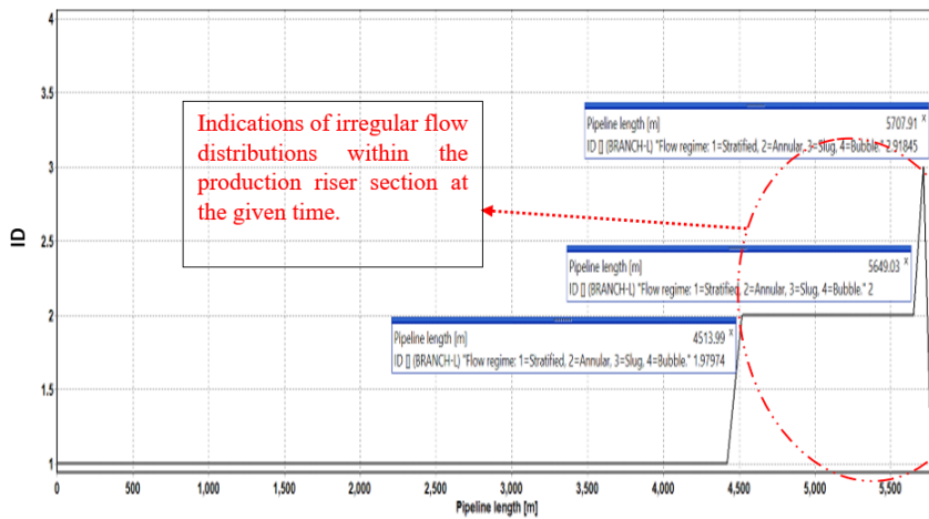
Figure 5. Flow regime distribution along pipe profile at 15000s
