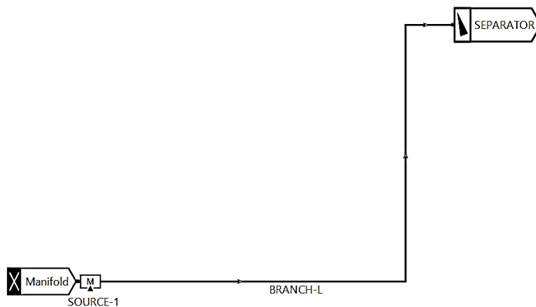
Figure 12: OLGA Base Case model
