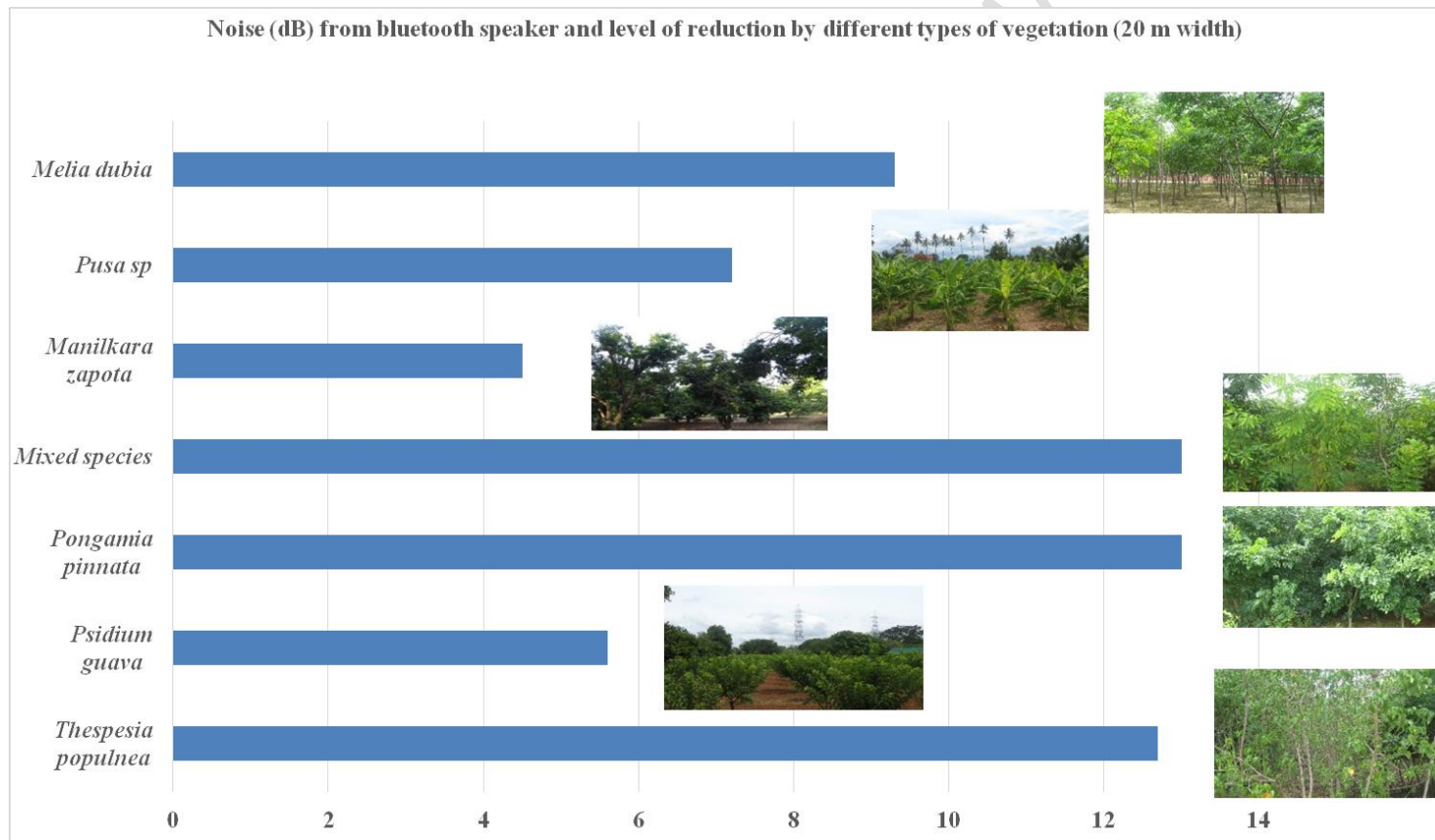
Fig. 1. Studies on noise level reduction by different types of vegetation when bluetooth speaker was played
