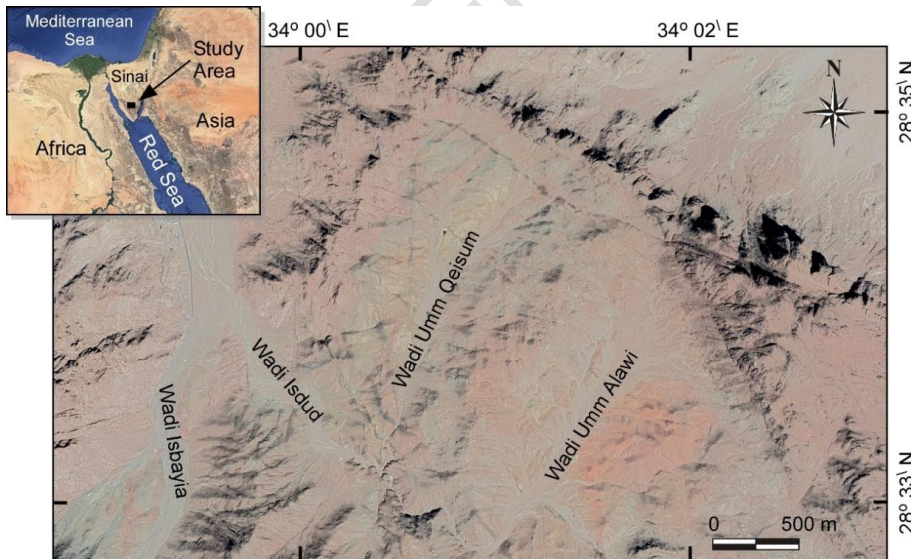
Fig. 1. Landsat image of the study area
