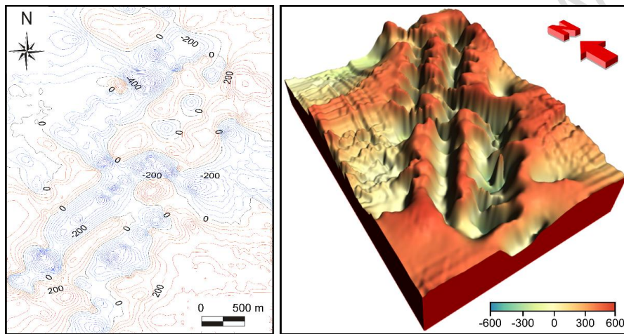
Fig. 4. Vertical magnetic gradient contour map (left) and 3D surface map (right)
