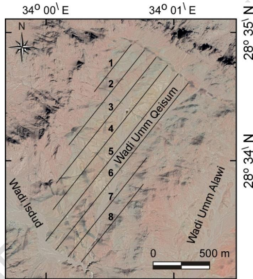
Fig. 3. Geophysical survey layout in the study area
