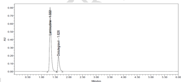
Figure 9. Thermal degradation chromatogram
