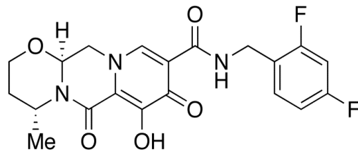
Figure 1. Structure of Dolutegravir
