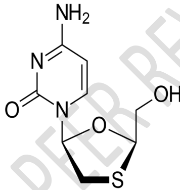
Figure 2. Structure of Lamivudine
