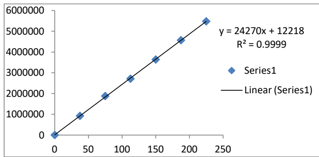
Figure 4. Calibration curve of Lamivudine
