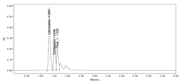
Figure 8. Peroxide degradation chromatogram
