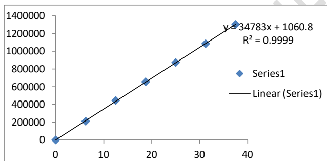
Figure 5. Calibration curve of Dolutegravir
