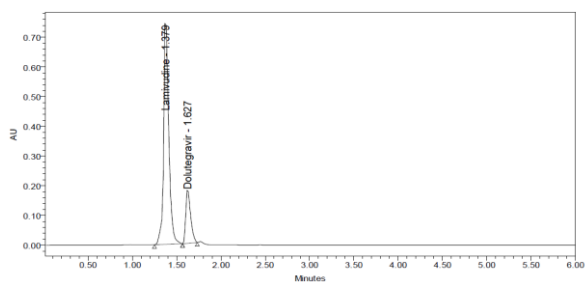
Figure 7. Base degradation chromatogram
