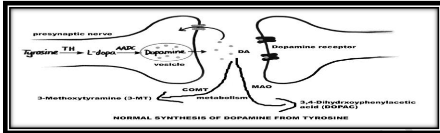
Picture.1 Normal synthesis of Dopamine from Tyrosine
