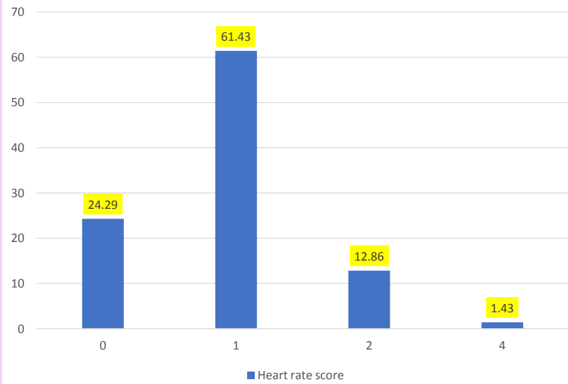
figure 8.Heart rate score
