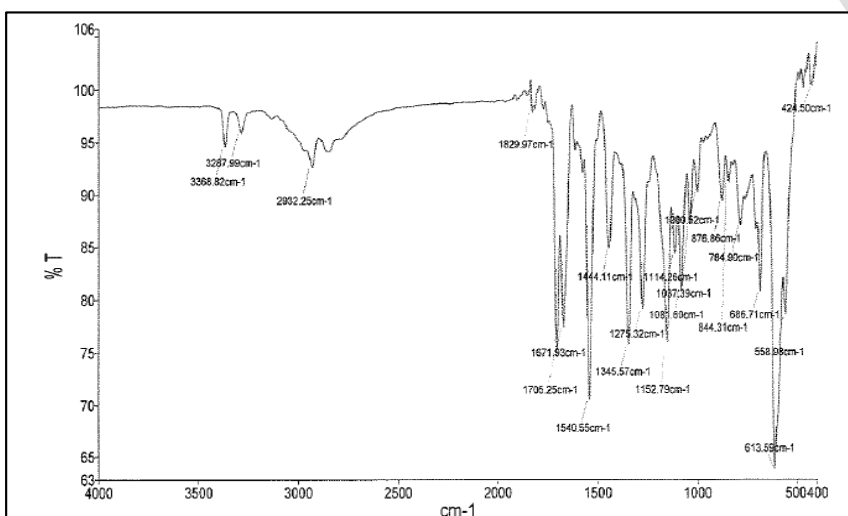
Figure 7: Fourier transform-infrared spectrum of Glimepiride-Polymer mixture (Initial)
