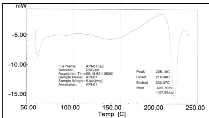
Figure 4: Differential Scanning Calorimetry (DSC) of Glimepiride
