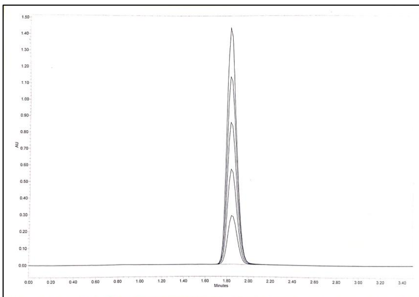
Figure 6: Linearity of Glimepiride by HPLC
