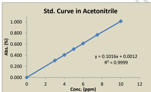
Figure 5: Standard curve of Glimepiride in Acetonitrile
