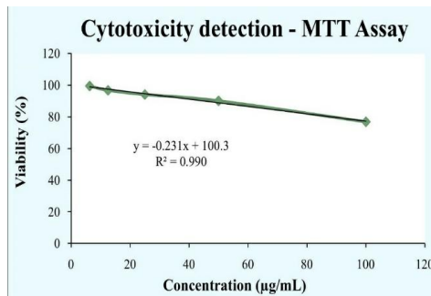
Fig.3.Cytotoxicity detection-MTT assay
