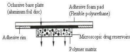
Figure 6: Micro reservoir Dissolution-Controlled TDDS
