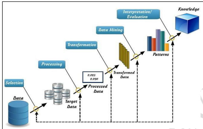
Figure 1: KDD Process.
