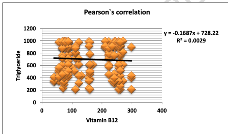
Graph– B. Scatter plot shows –ve correlation of triglycerides and vitamin B 12
