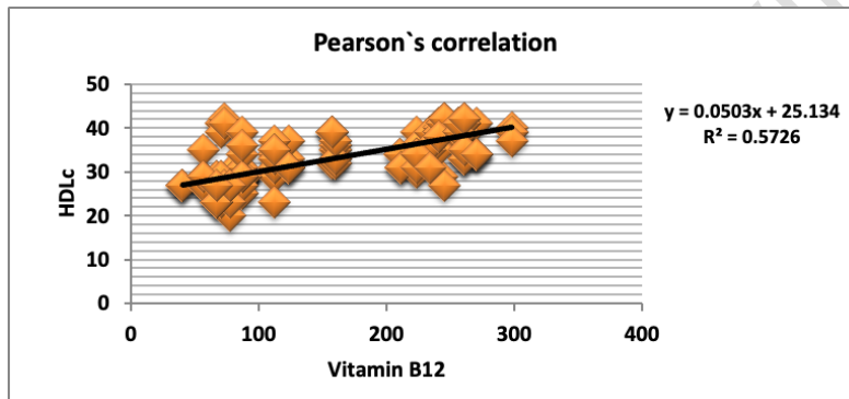
Graph – D. Scatter plot showing +ve correlation of HDLc and vitamin B 12
