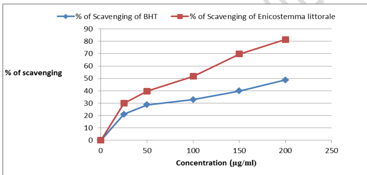
Fig. 1: The regression curve of DPPH Radical Scavenging Activity of Encostemma littorale
