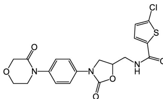
Figure 1: Structure of Rivaroxaban (3)
