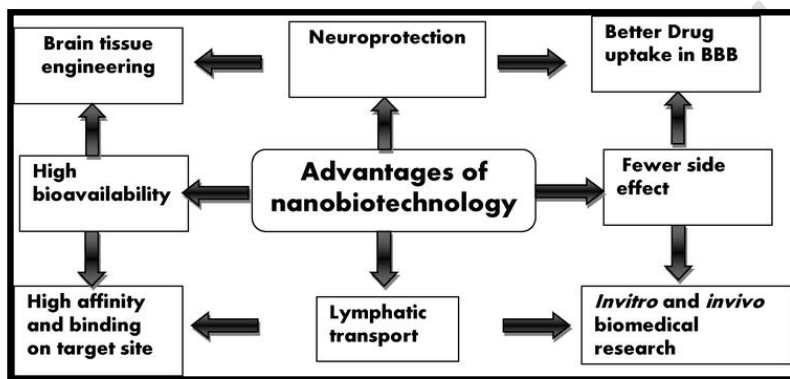
Figure 1: Nanobiotechnology Advantages [26].
