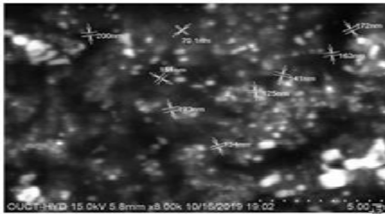
Fig 5: SEM images of the biosynthesized of AuNPs s
