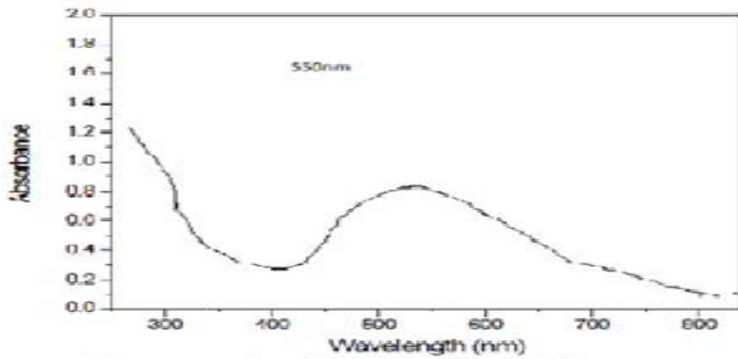
Fig 3: UV-VIS absorption spectra of synthesized Au NPs
