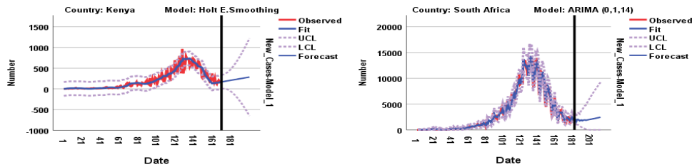
Figure 3. The fitting models and forecasts graphs of COVID-19 new cases for the countries from February 14 to September 06, 2020.
