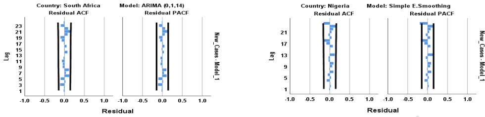
Figure 2. The graphs of ACF and PACF residuals
