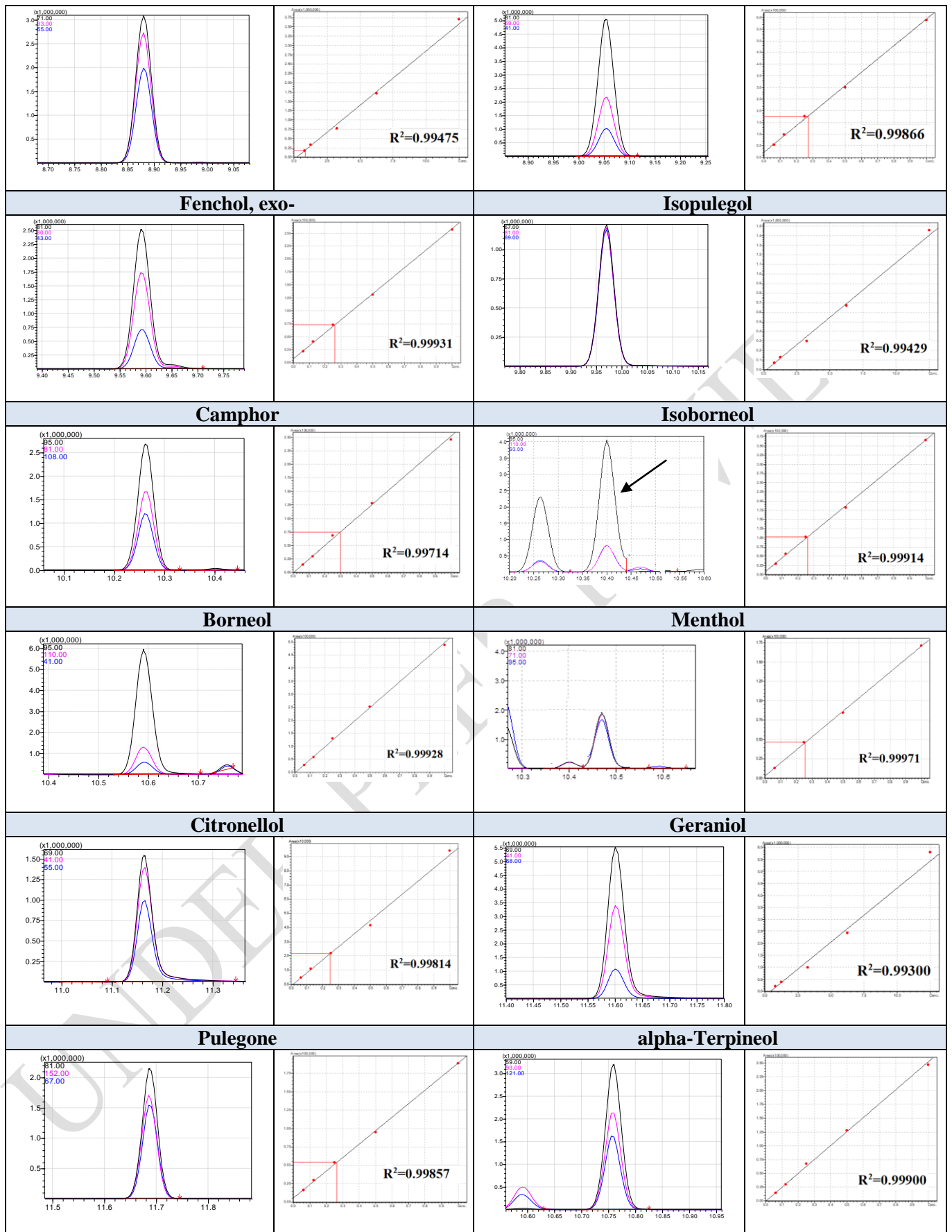
Figure 1-2. Typical chromatograms and calibration curves of the standard solutions for terpene testing
