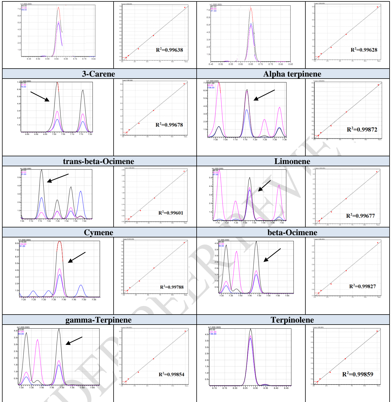
Figure 1-1. Typical chromatograms and calibration curves of the standard solutions for terpene testing
