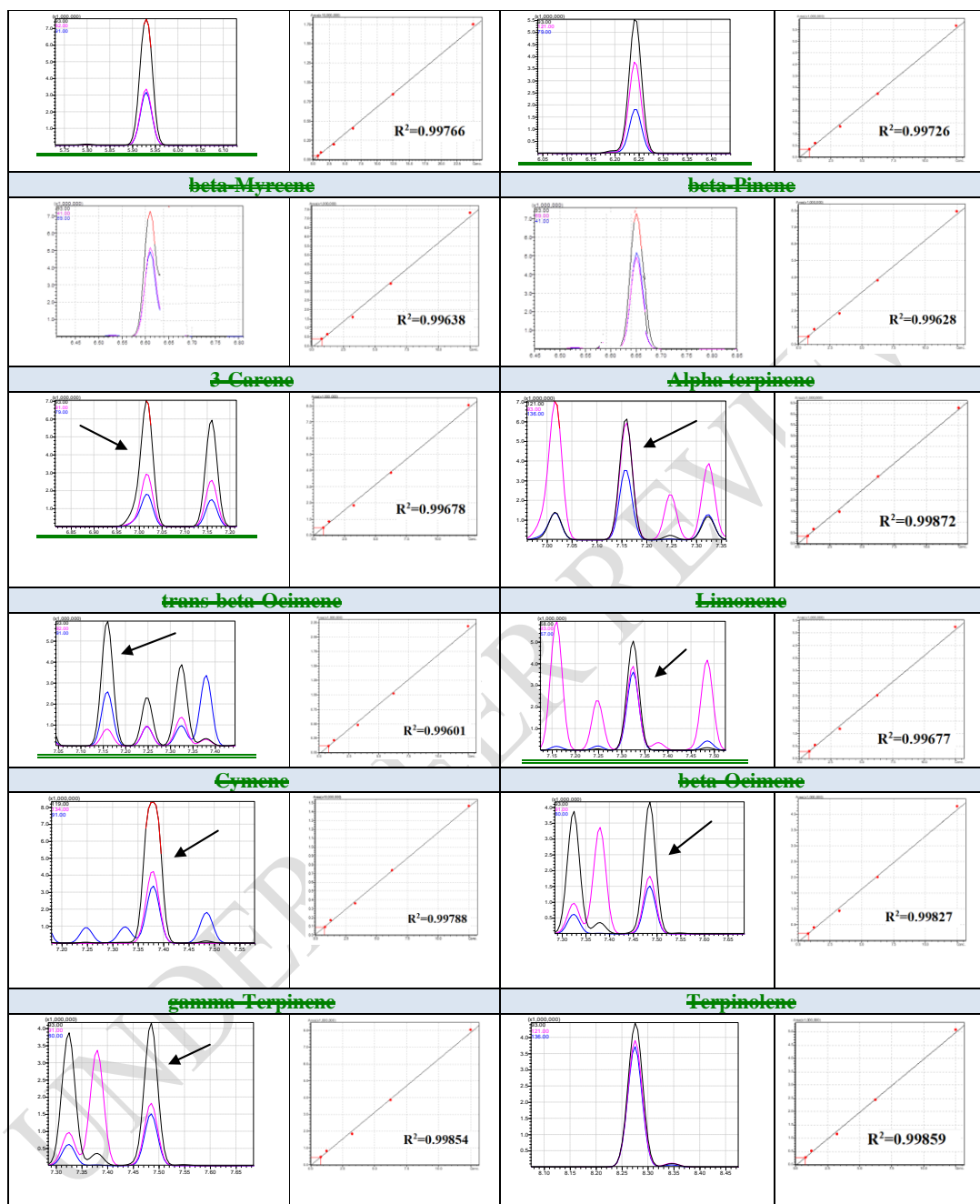
Figure 1-1. Typical chromatograms and calibration curves of the standard solutions for terpene testing
