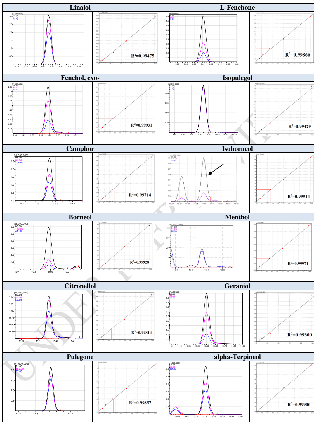
Figure 1-2. Typical chromatograms and calibration curves of the standard solutions for terpene testing
