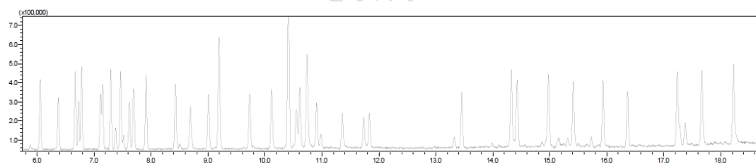
Figure 2. Typical chromatogram for chromatographic separation of terpenes
