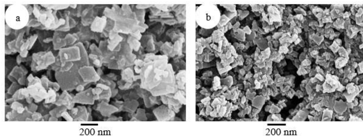
Fig. 5. SEM images of UiO-66(Zr)-green (a) and 10SA/UiO-66(Zr) (b).
