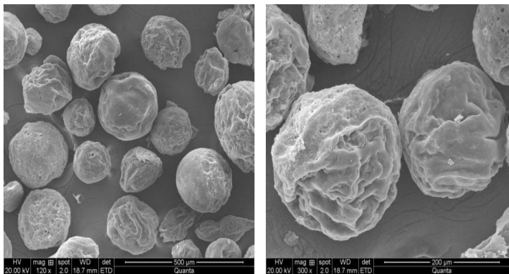
Figure 3: SEM photograph of microspheres at different magnifications
