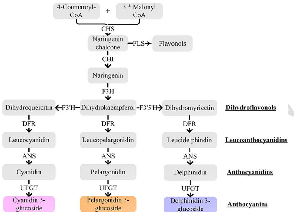
Fig: 3 Biosynthesis of anthocyanin [Source: https://www.frontiersin.org/files/Articles/308869/fchem-06-00052-HTML/image_m/fchem-06-00052-g004.jpg ]
