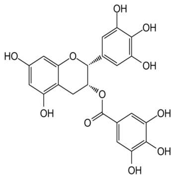
Fig: 4 chemical structure of EGCG [source: https://5.imimg.com/data5/RG/NJ/MY-8206856/egcg-epigallocatechin-gallate-500x500.png ]
