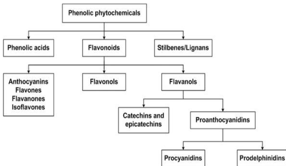
Fig:2- anthocyanin [Source: https://www.intechopen.com/books/flavonoids-from-biosynthesis-to-human-health/antioxidant-capacity-of-anthocyanin-pigments ]
