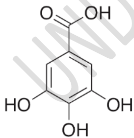
Fig:5 gallic acid. [source: https://lktlabs.com/product/gallic-acid/ ]
