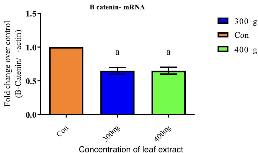
Figure-3 Effect of Aegle marmelos leaf extract on B- Catenin mRNA expression in MCF-7 cells.
