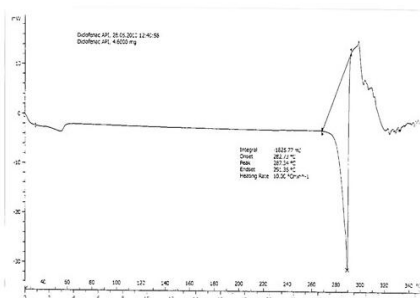
DSC thermogram of Diclofenac Sodium
