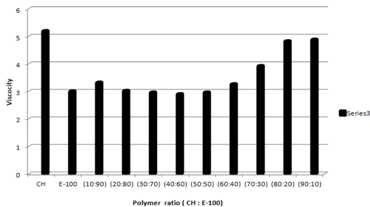
Figure 3 Viscosity of different polymer solution
