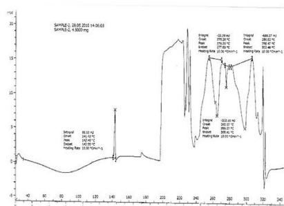
DSC thermogram of Eudragit L100
