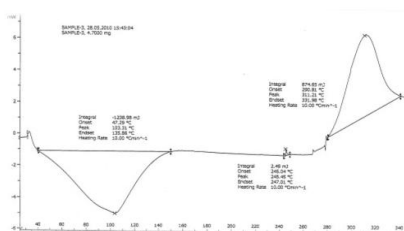
DSC thermogram of Chitosan
