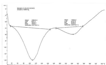
DSC thermogram of IPEC 40:60
