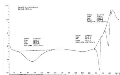
DSC thermogram of IPEC 40:60 + Diclofenac Sodium
