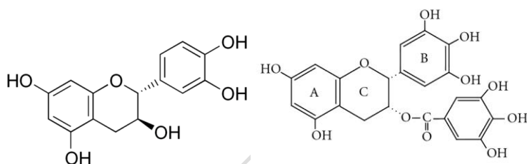
Figure 2 Chemical structure of Catechin
