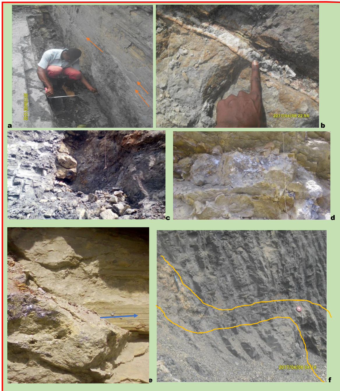
Figure 11: Vein mineral of the study area, (a) calcite and quartz minerals alignment parallel to the vein walls, as indicated by the arrow, scale: 2.75"x 3.16" (b) Quartz vein growing inward from the wall rock, scale: 2.76"x 3.65" (c, d) nearly vertical siderite and Pb-Zn vein deposits respectively, scale: 1.99"x 3.54" (e) Copper vein with slickenlines at Enyigba, scale: 3.47"x 3.15" (f) Curved Pb-Zn vein at Izzi, scale: 3.4"x 3.8"
