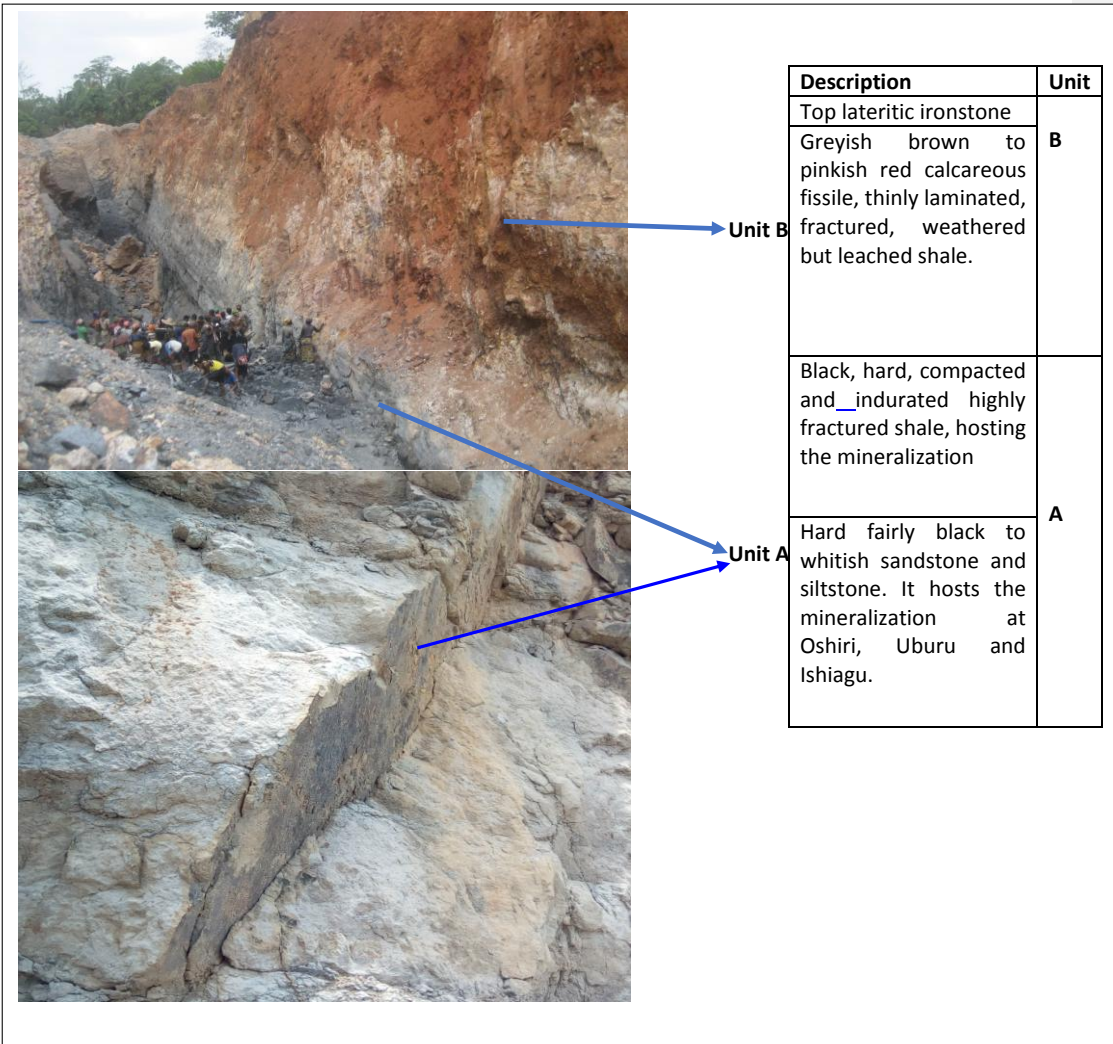
Figure 10: Lithologies hosting the mineralization, see text for description. Picture scale: 2.99” x 3.98”
