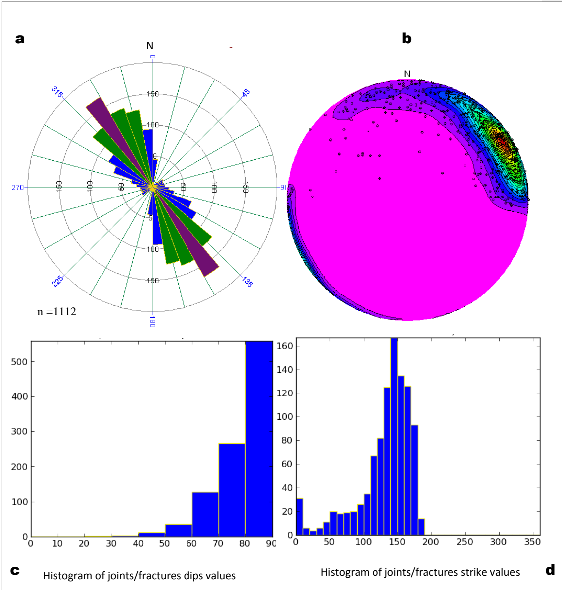
Figure 9: Composite J joints and F fractures diagrams. The true joints are >70^{\circ} dips, 30-60^{\circ} dips are fractures (a) Composite rose diagram of joints and fractures, (b) Composite Stereogram showing poles to joint and fracture planes, lower hemisphere projection, (c) Composite dip Diagram of joints and fractures (d) Composite strike frequency diagram
