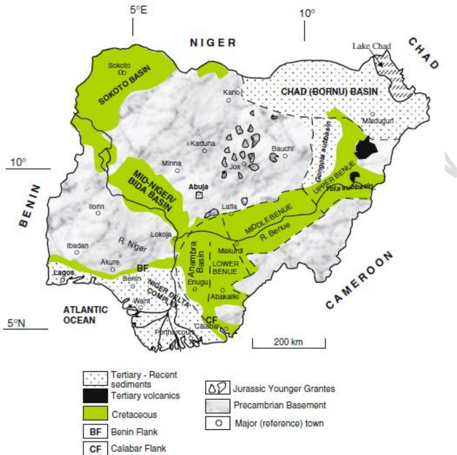
Figure 3: Geological Map of Nigeria showing (a) Romanche, Chain and Charcot extension fractures zones from Mid-Atlantic ridge to the Nigerian coastline, Benue Trough, Basement Complex and Volcanics, while (b) majorly shows the arbitrary partitioning of Benue Trough with other sedimentary basins, Basement Complex and Younger Granites (after Whiteman, 1982; Obaje, 2009).
