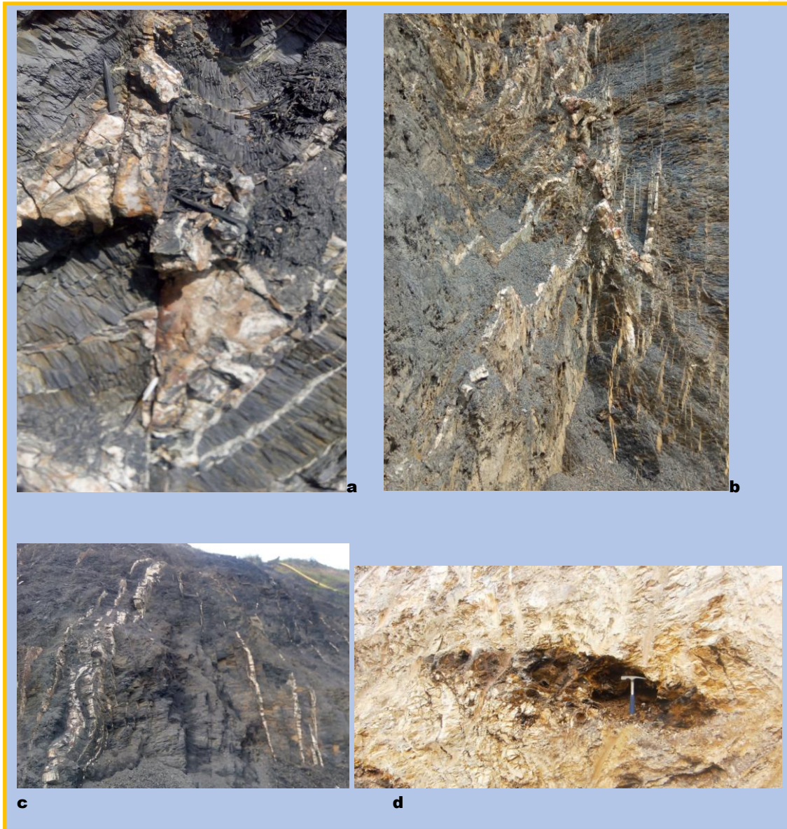
Figure 12: (a) Faulted vein deposit, scale: 4.49" x 3.07". (b) Tight folded vein deposit, scale: 4.45" x 3.21". (c) Anticlinal folded vein deposit, 2.27" x 3.08". All were observed at Enyigba axis. This indicates that faults and folds also control the mineralization. (d) Concordant type of vein occurrence, ellipsoidal in shape, scale: 2.06" x 3.97"
