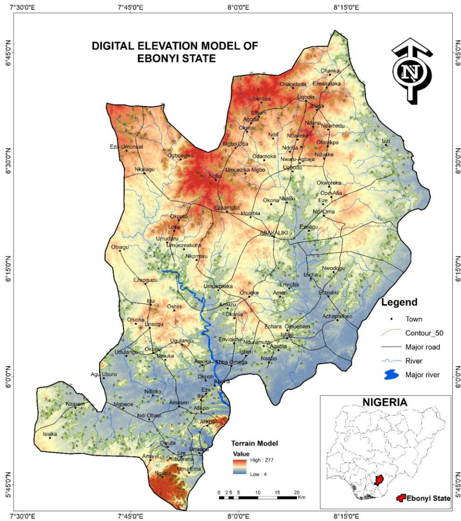
Figure 1: Topographic Map of the Study Area
