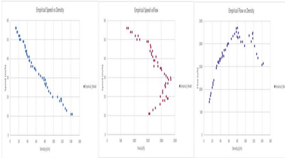
Figure 5: Speed-Flow-Density Curves for the Empirical Data
