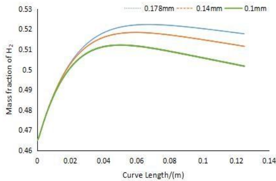
Fig. 15. Mass distribution curve of hydrogen in the anode runner
