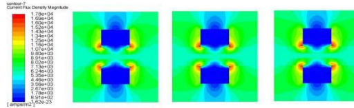
Fig. 13. Current density distribution at the intermediate section
