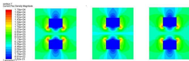
Fig. 7. Distribution of current density in the middle of different GDL thicknesses
