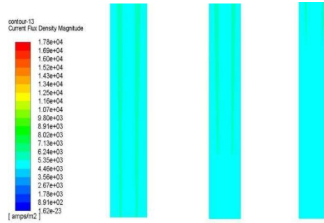
Fig. 8. Distribution of current density on the proton exchange membrane near the inlet position
