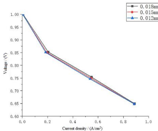
Fig. 12. Polarization curves of fuel cells with different catalytic layer-CL thicknesses
