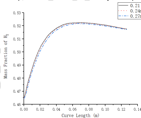
Fig. 4. Hydrogen distribution in the anode runner
