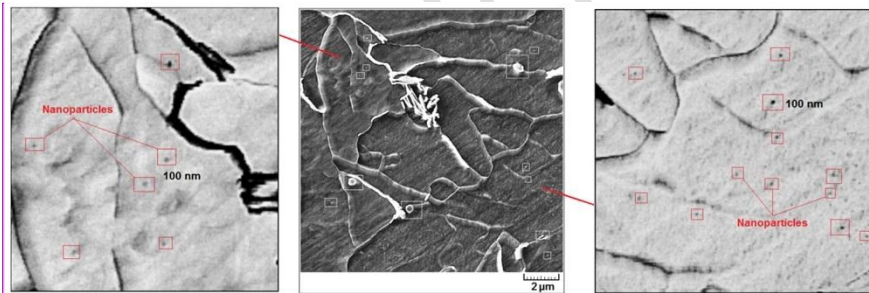
Figure 7. Vanadium in the weld metal
