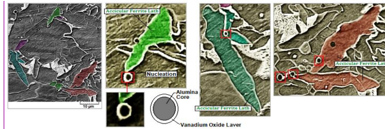
Figure 12. Formation of acicular ferrite by a shell of the Core/ Shell structure
