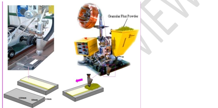
Figure 4. Experimental setup
