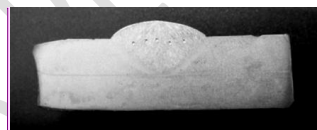
Figure 5. Weld melted zone
