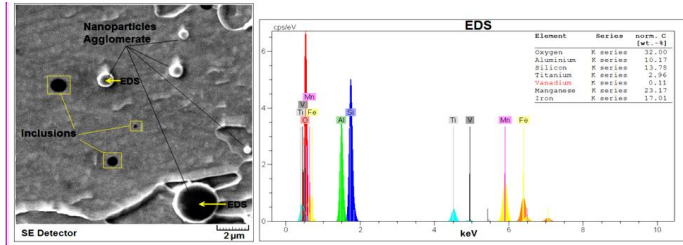
Figure 6. SEM micrograph of weld metal with its EDS
