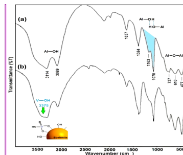
Figure 3. FTIR spectra of synthesized (a) nano-boehmite (b) and BNV
