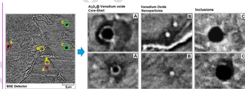
Figure 9. BSE micrograph of the melted zone
