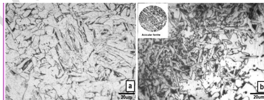
Figure 11. Optical micrographs of the melted zone microstructure at various thicknesses of BNV (a) 0.0 mm (b) 1.0 mm
