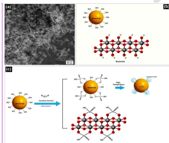
Figure 2. Structure of boehmite nanoparticles
