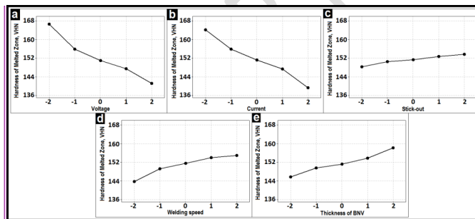
Figure 10. Main effects of input parameters on HMZ
