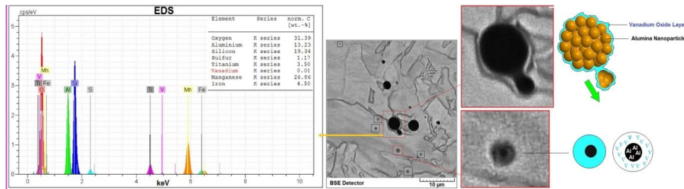
Figure 8. Core-shell structure of boehmite and vanadium nanoparticles
