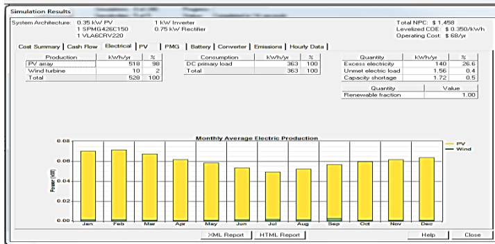
Fig. 14. Monthly average electric production
