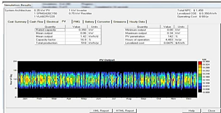
Fig. 15. Photovoltaic system simulation output
