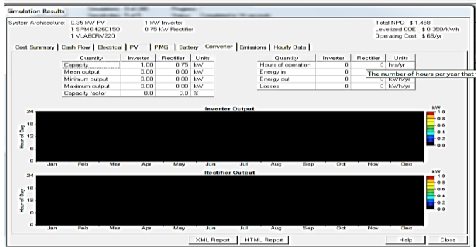
Fig. 18. Inverter simulation output
