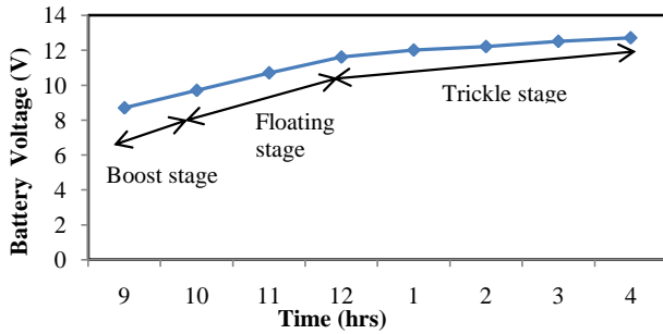
Fig.8. Battery voltage against time
