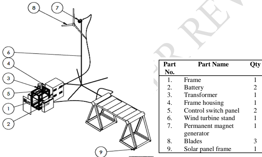
Fig. 5: General layout of the whole system
