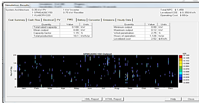
Fig. 16. Wind turbine simulation output
