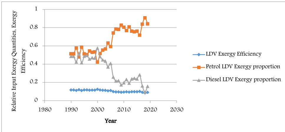
Figure 3. Effects of Relative Input Exergy Quantities on LDV Exergy Efficiency
