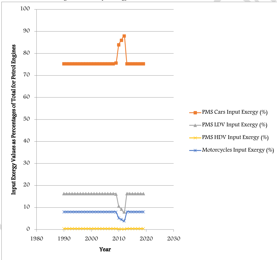
Figure 2. Petrol Engines Percentage Exergy Utilisations
