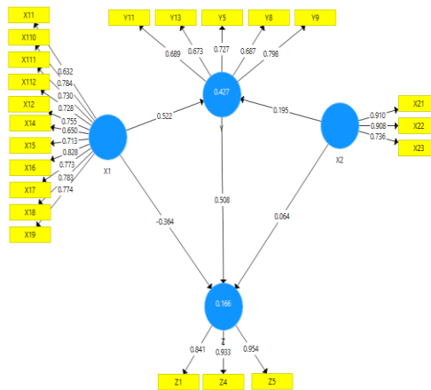
Source: Processed Data (2021) Figure 1. Loading Factor Model
