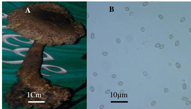
Fig. 1. A: Carpophore of Psathyrella caput-medusae and B: Spores (x400)
