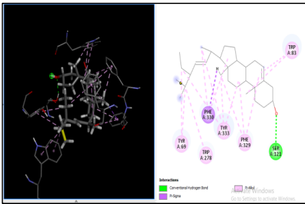
a) Stigmasterol – 11.9
