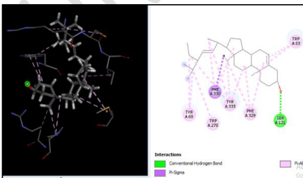
c) Stigmasterol – 8.4
