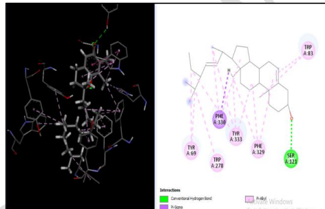
d) Tocopherol – 9.9
