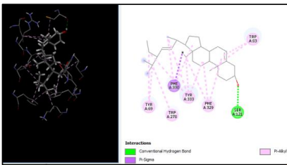
a) Stigmasterol – 9.6
