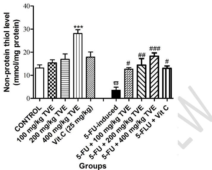
Figure 3: Effect of T. vulgaris extract (TVE) on the non-protein thiol level in the penile of normal and 5-fluorouracil (5-FLU)-induced oxidative stressed male rats
