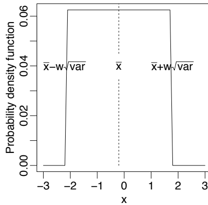
font size Figure 5: Probability density function of the uniform distribution. “var” denotes the third variance of the data.
