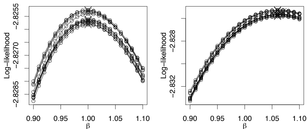
font size ( Figure 1: Relationship between \beta and log-likelihood in light of future data. “x” denotes the maximum point.
