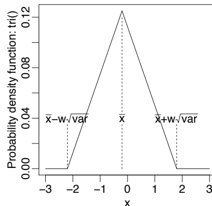
font size ( Figure 2: Probability density function of the triangular distribution. “var” denotes the third variance of the data.
