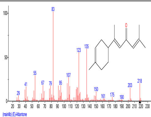
Fig. 2k. Mass spectrum of (E)-Atlantone structure.
