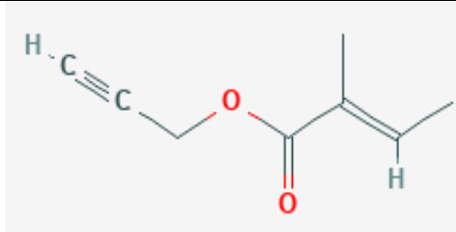
Fig. 2n. Structure of Prop-2-ynyl (E)-2-methylbut-2-enoate.
