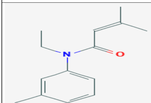
Fig. 2q. Structure of But-2-enamide, N-ethyl-N-(3-methyl phenyl)-3-methyl-
