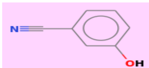
Fig. 2j. Structure of Benzonitrile, 3-hydroxy
