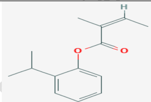
Fig. 2l. Structure of Cumenyl angelate, o-
