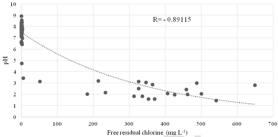
Figure 5. Correlation between pH values and free residual chlorine from sanitary effluents after treatment.
