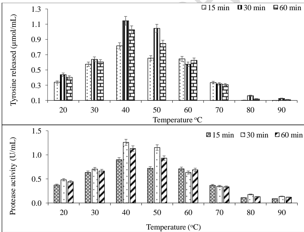
Figure 2: Stability of protease produced by Alcaligenes faecalis P2 at different temperatures indicated by released tyrosine and protease activity.
