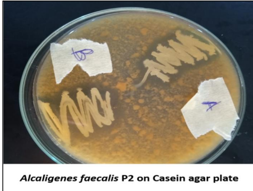
Figure 1: Casein Agar Plate screening of the protease-producing bacterium Alcaligenes faecalis P2.
