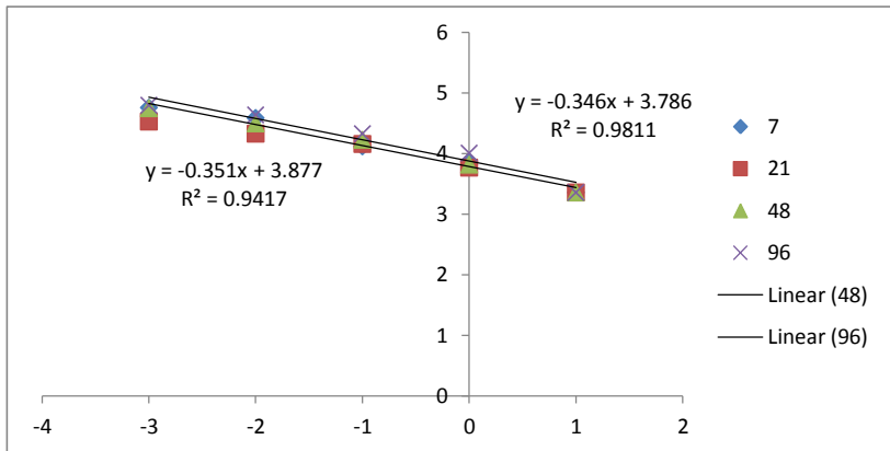
Figure 3: Toxicity of Candida haemulonii (Sophorolipid) against Nitrobacter sp.
