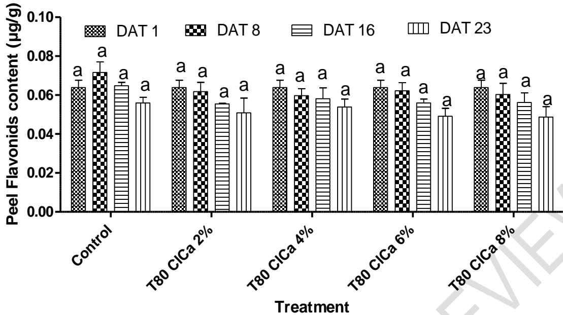
Fig. 8a: Evolution of the flavonoid content in the peel
