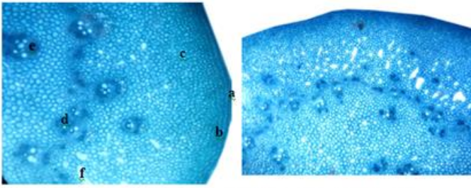
Plate 5: Transverse sections of the petiole of Anthocleista djalonesis A.Chev x10. a: Epidermis; b: Collenchyma; c: Sclerenchyma; d: Vascular bundle; e: Medullary bundle f: Intercellular space
