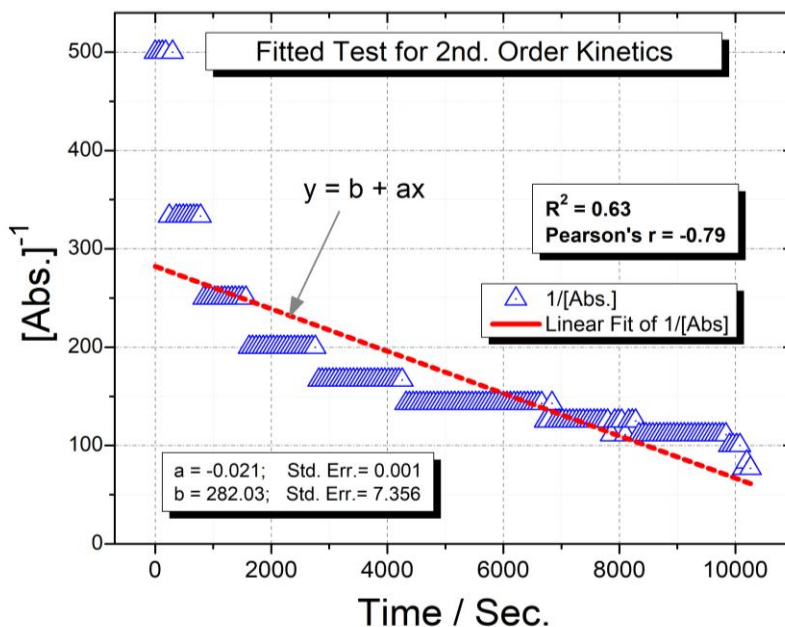
Figure 8(b): Fitted Test for Second - Order Kinetics
