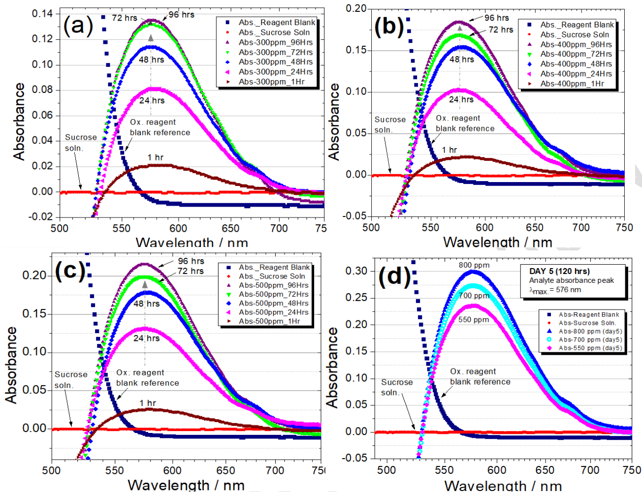
Figure 4: Dependence of the Cr(III) analyte peak on reaction time and the sucrose substrate concentration
