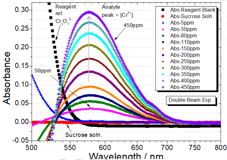
Figure 2: Absorbance spectra of the analyte peak of the standards
