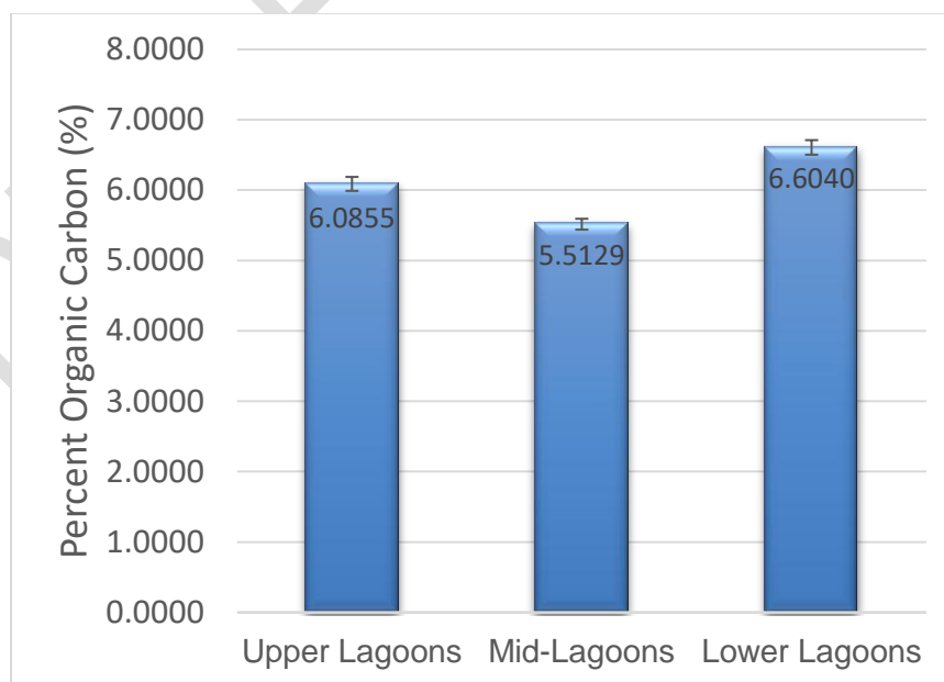
Figure13: Histogram chart comparing the percent OC obtained from upper, mid-, and lower sewage treatment plant lagoons near the banks of River Njoro
