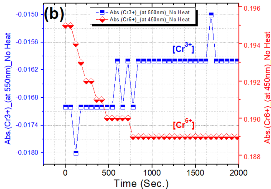
Figure 9(b): Kinetic profile of the Cr(VI) reactant and Cr(III) product absorbance data recorded during sucrose oxidation under room temperature conditions for the first 2000 s
