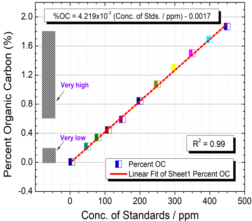
Figure 11: Conversion chart for the estimation of %OC in soil samples
